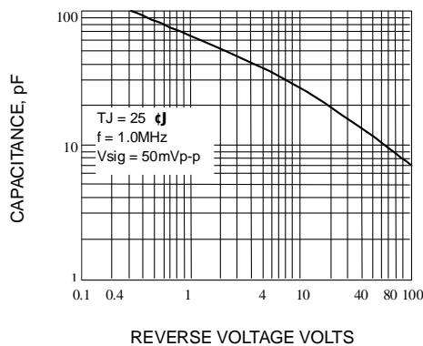
Fig. 4-TYPICAL JUNCTION CAPACITANCE
